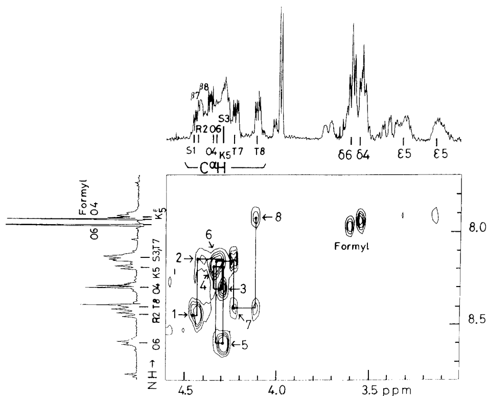
Fig. 4. ^1\text{H} -ROESY map showing the cross-peaks in \text{X-CH}\alpha and \text{Y-NH} correlated region. The number assigned to each arrow indicates the position i of the \text{C}\alpha\text{H}(i) in the amino acid sequence. The correlations for the following \text{X-Y} couples \text{S}_1\text{-R}_2 (arrow 1), \text{R}_2\text{-S}_3 (arrow 2), \text{S}_3\text{-O}_4 (arrow 3), \text{O}_4\text{-K}_5 (arrow 4), \text{K}_5\text{-O}_6 (arrow 5), \text{O}_6\text{-T}_7 (arrow 6), \text{T}_7\text{-T}_8 (arrow 7) and \text{CH}\alpha(\text{T}_8)\text{-NH}\epsilon(\text{K}_5) (arrow 8) allow a distinction between \text{Ser}_1/\text{Ser}_3 , \text{Orn}_4/\text{Orn}_6 and \text{Thr}_7/\text{Thr}_8 spin systems. Amino acid residues are represented in the one-letter code
