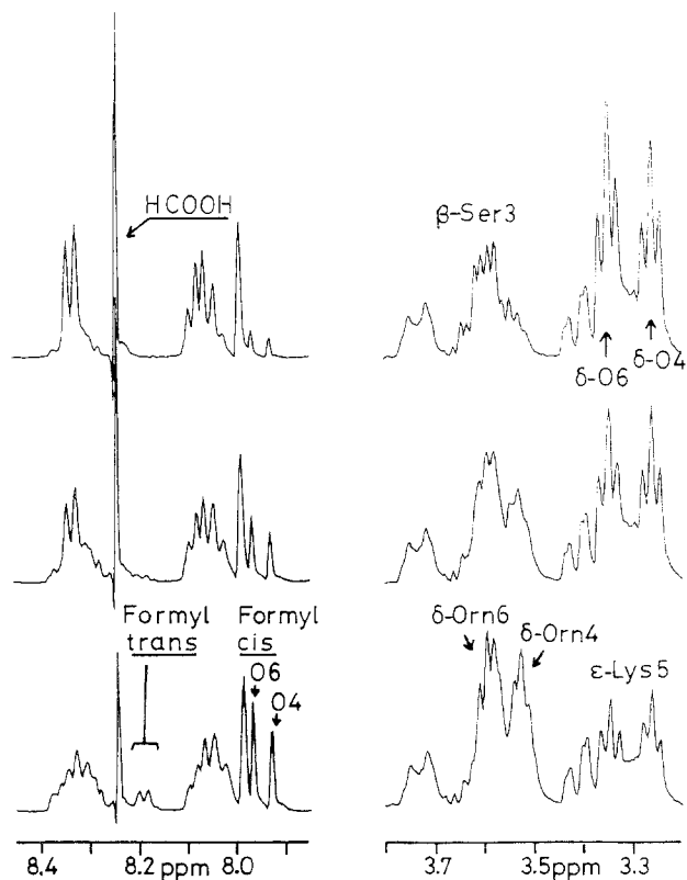
Fig. 5. Evolution of the formyl and \text{CH}_2\delta proton resonances at different hydrolysis stages
