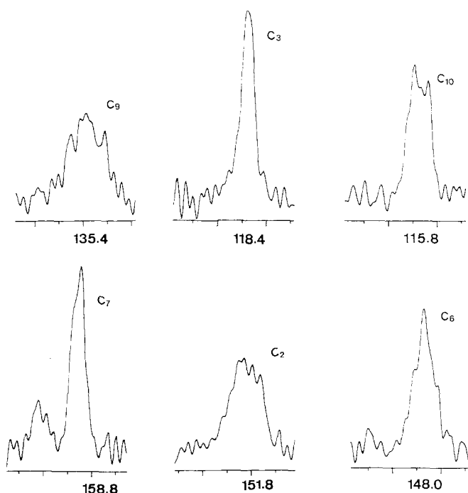
Fig. 7. Assignment of the quaternary carbon atoms of the chromophore of pyoverdine Pa A from their long-range coupling constants at 100 MHz
