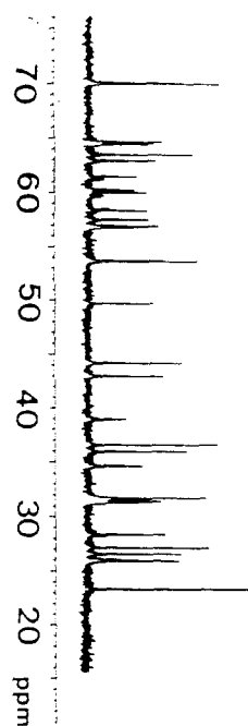
Fig. 8. ^1\text{H} - ^{13}\text{C} heteronuclear correlation NMR spectrum of pyoverdine Pa A determined in ^2\text{H}_2\text{O} with sodium trimethylsilyl( ^2\text{H}_6 )propane sulfonate as an internal standard
